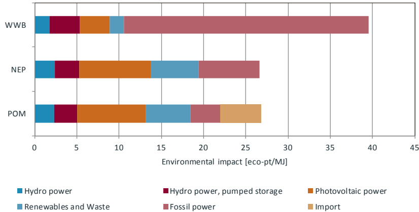
Fig. 3.2 Environmental impacts of the electricity mix per scenario in [eco-points/MJ]
