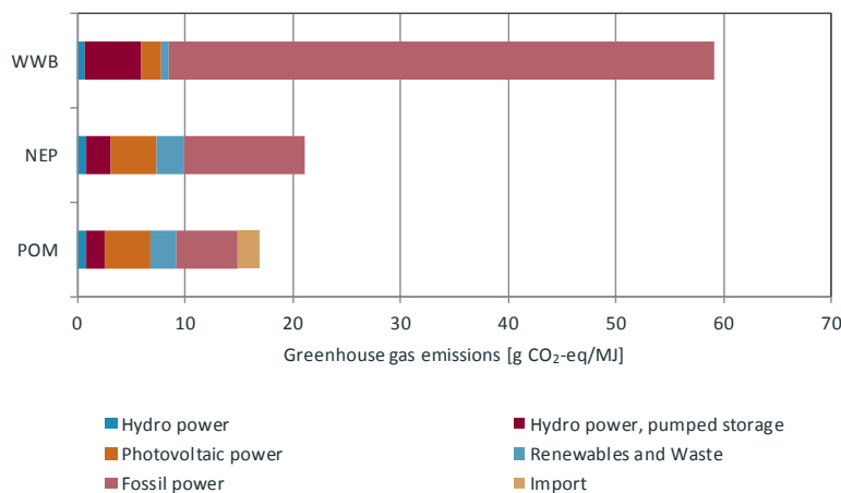
Fig. 3.1 Global warming potential of the electricity mix per scenario in [g CO 2 -eq/MJ]
