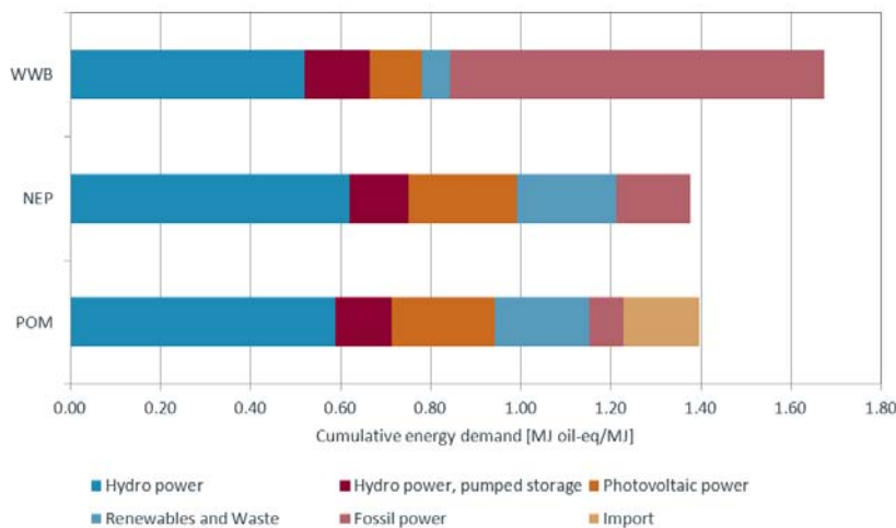
Fig. 3.3 Cumulative energy demand of the electricity mix per scenario in [MJ oil-eq/MJ]
