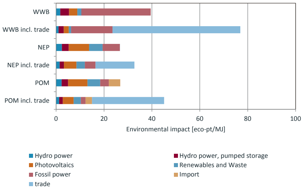
Fig. Z. 5 Environmental impacts of of the electricity mixes, with and without trade, ecological scarcity method 2006
