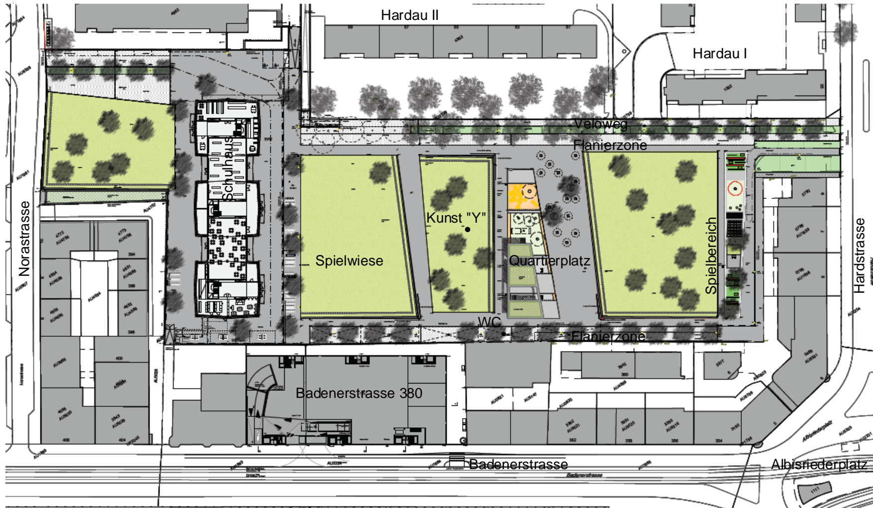
Situationsplan Hardaupark
